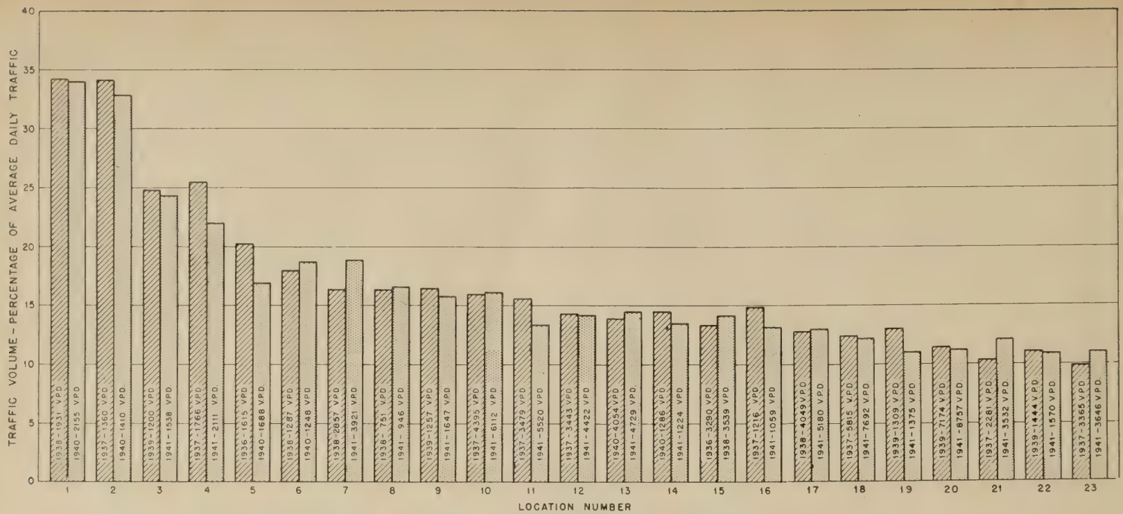
Figure 52.—Comparison of thirtieth highest hourly volumes for two different years at identical locations.
